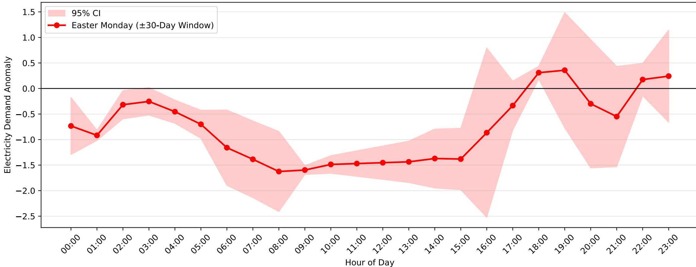
Adamstown Demand Anomaly: Easter Monday (2016-2017, \pm 30 -Day Window)
